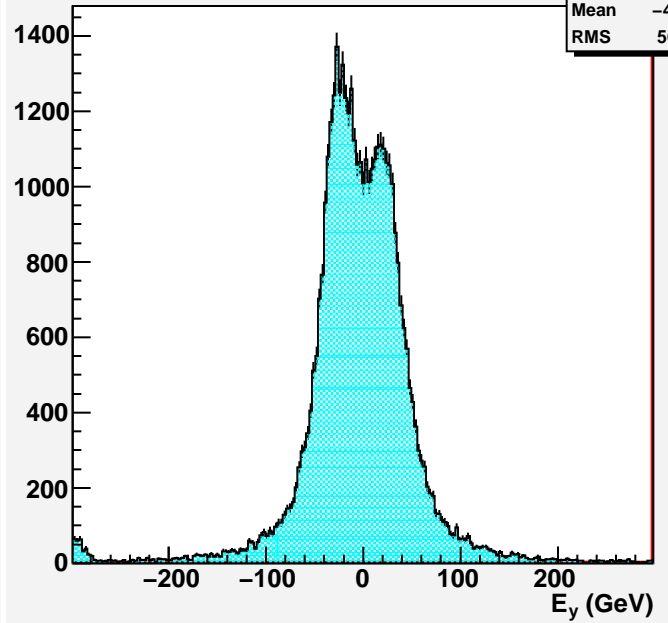
EF Missing E_y
