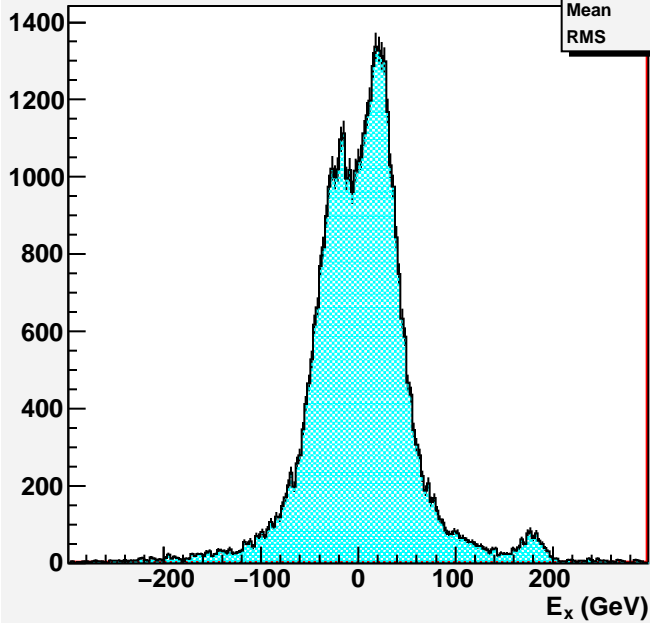
EF Missing E_x
