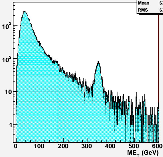
EF |Missing E_T |
