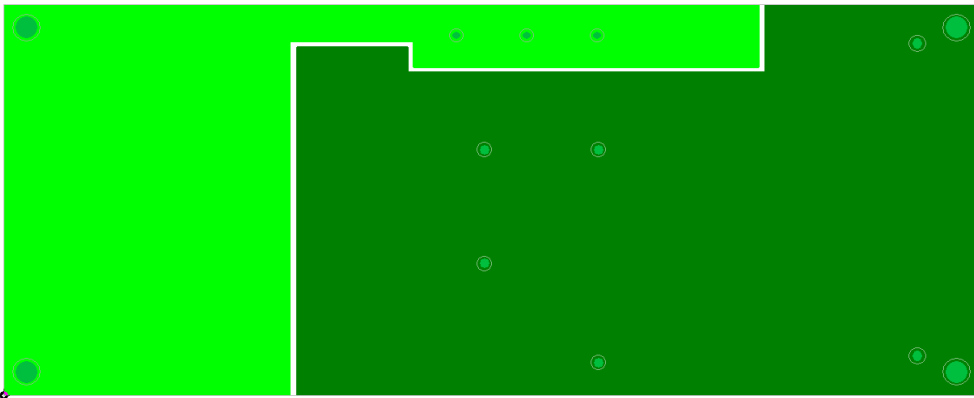
LAYER: Inner3 VSS/GND
