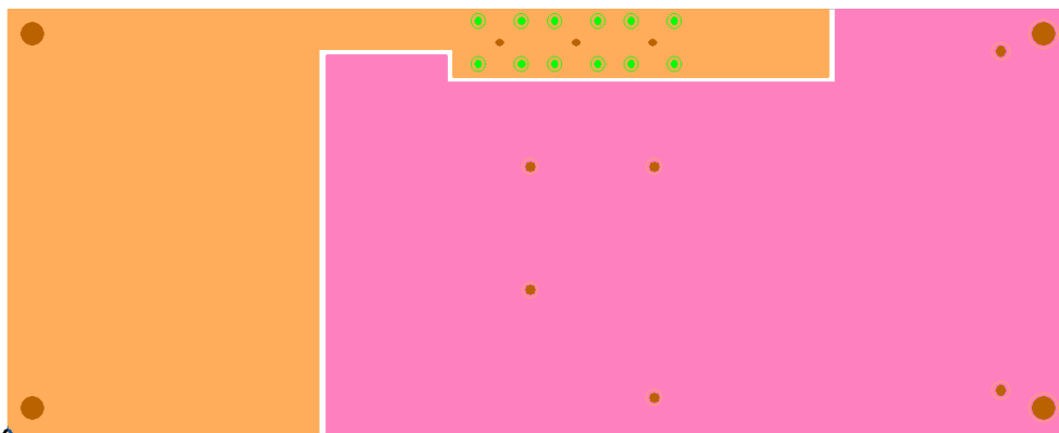
LAYER: Inner 4 VDD/VDDD
