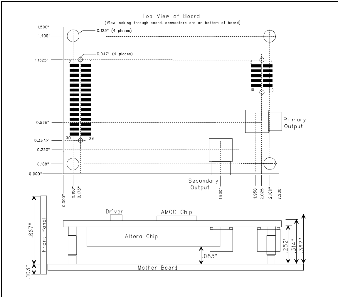
Figure 2 – Mechanical Layout
