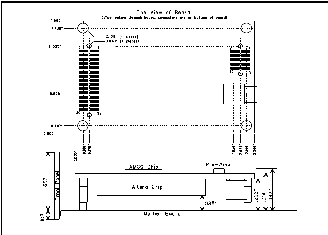
Figure 2 - Mechanical Dimensions
