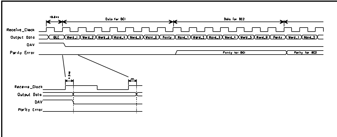
Figure 1 - Receive Timing
