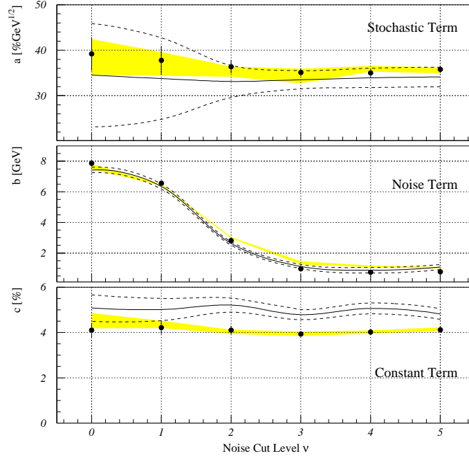
Figure 19: Contributions to the relative energy resolution, as fitted using eq.(6), as function of the noise cut \nu . The full circles are experimental data, the shaded area indicates the GEANT3 values and their errors, and the solid line represents the GEANT4 values, with the dotted lines showing the corresponding error.
