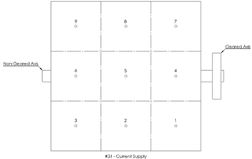
Aluminum Plate Temperature Probe Location
