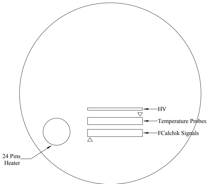
Top Plate viewed from above
