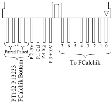
FCalchik Signal Connector
